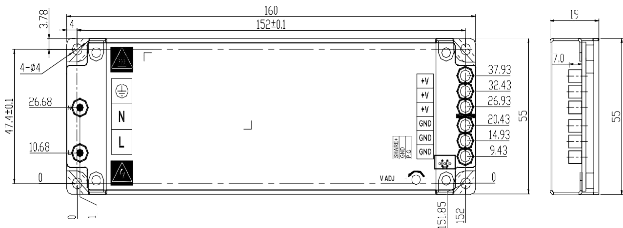
Dimensions and mounting holes - terminal coordinates
